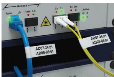
Flexible ID-tape
